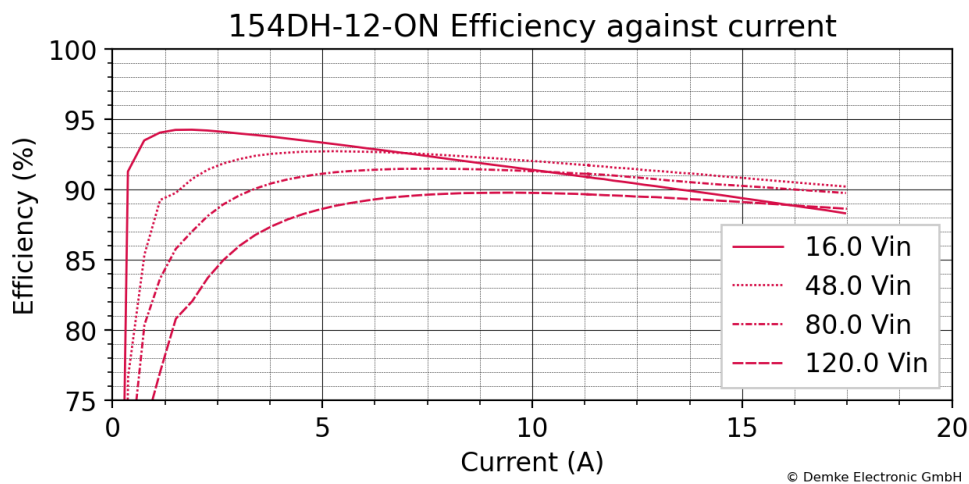
Figure 2 Efficiency in the constant voltage range of the DC-Transformer 154DH-12-ON
