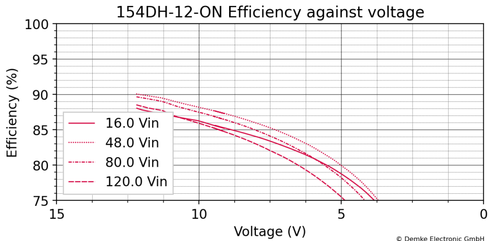
Figure 3 Efficiency in the constant current range of the DC-Transformer 154DH-12-ON
