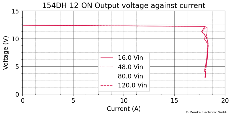
Figure 1 Voltage against current of the DC-Transformer 154DH-12-ON
