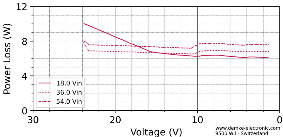
Figure 5: Power Loss over voltage of the DC-Transformer 256-24-SD
