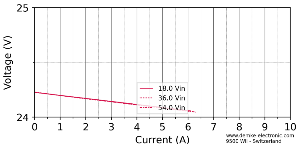
Figure 6: Voltage in CV-mode of the DC-Transformer 256-24-SD
