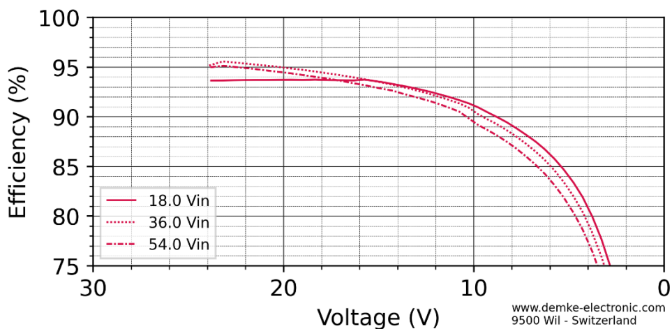
Figure 3 Efficiency in the constant current range of the DC-Transformer 256-24-SD
