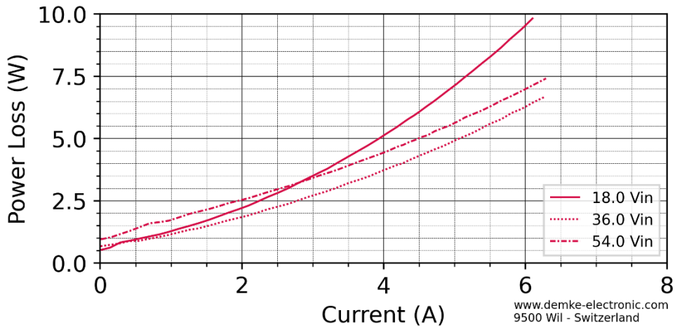
Figure 4: Power Loss over current of the DC-Transformer 256-24-SD
