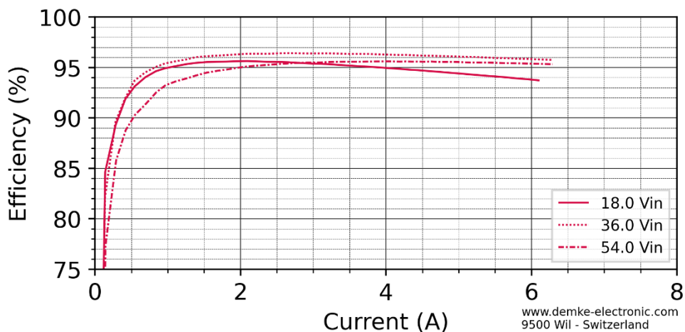
Figure 2 Efficiency in the constant voltage range of the DC-Transformer 256-24-SD
