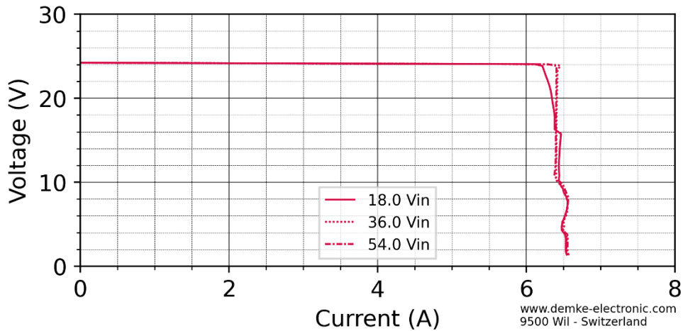
Figure 1 Voltage against current of the DC-Transformer 256-24-SD
