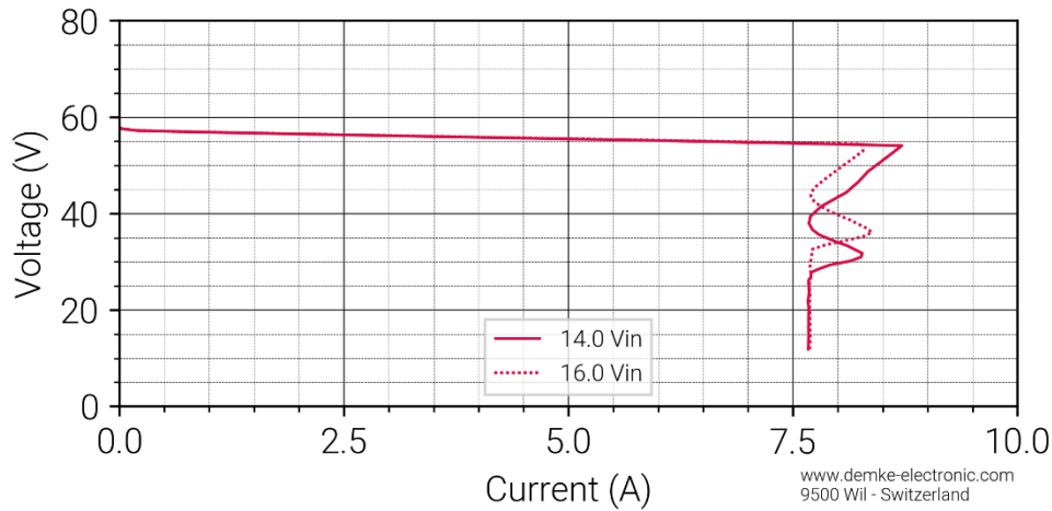
Figure 1 Voltage against current of the DC-Transformer 729-57-SD
