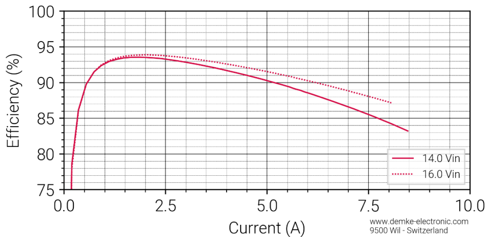
Figure 2 Efficiency in the constant voltage range of the DC-Transformer 729-57-SD
