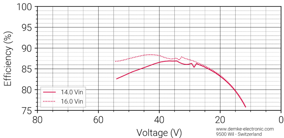
Figure 3 Efficiency in the constant current range of the DC-Transformer 729-57-SD
