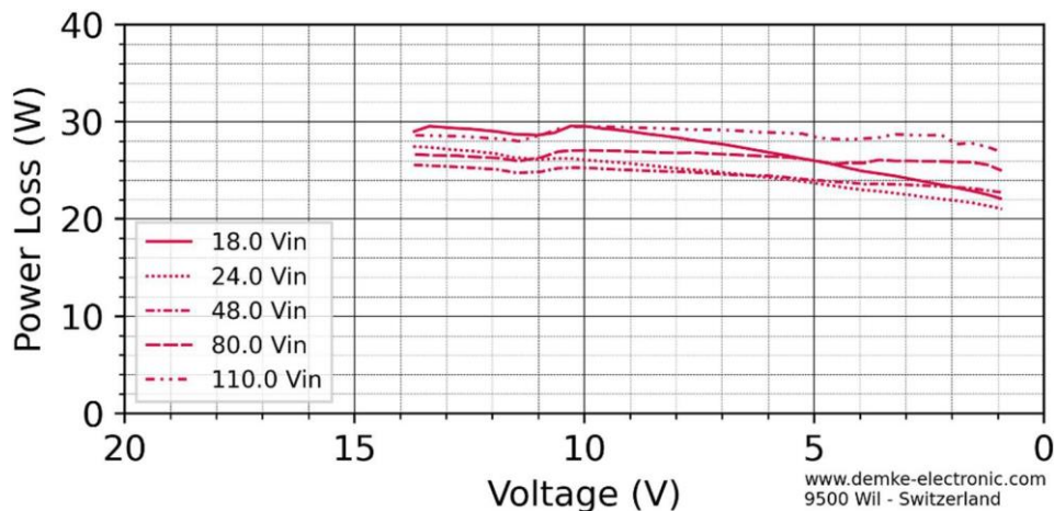
Figure 6: Voltage in CV-mode of the DC-Converter
