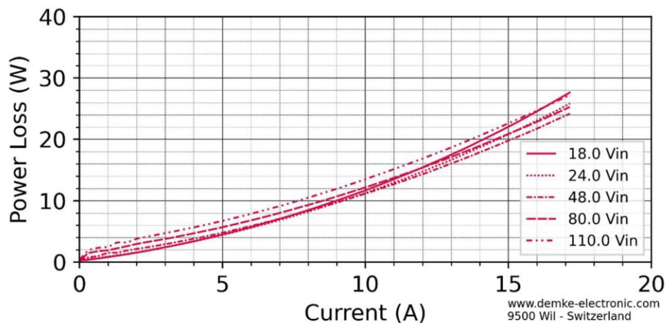
Figure 4: Power Loss over current of the DC-Converter
