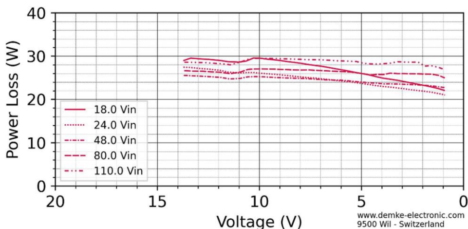
Figure 5: Power Loss over voltage of the DC-Converter
