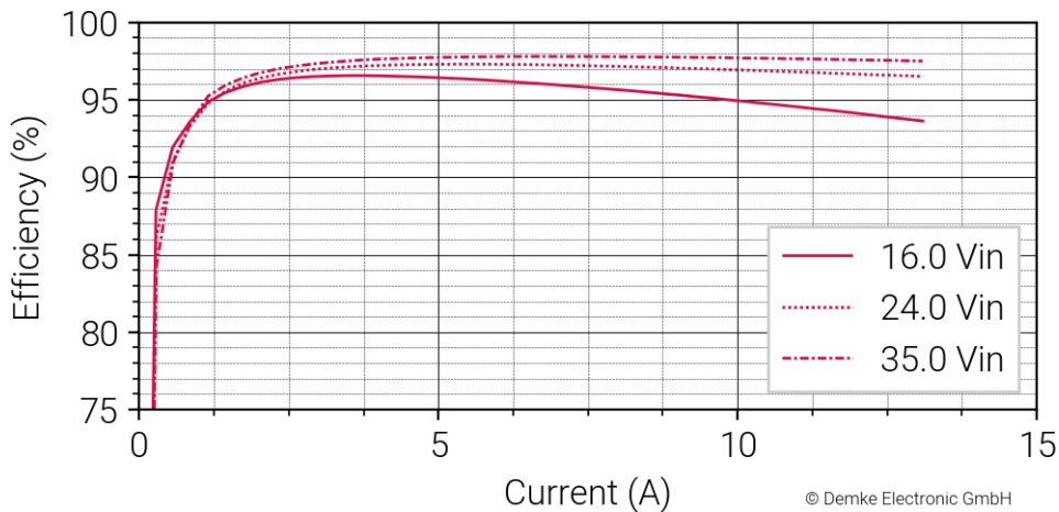
Figure 2 Efficiency in the constant voltage range of the DC-Converter
