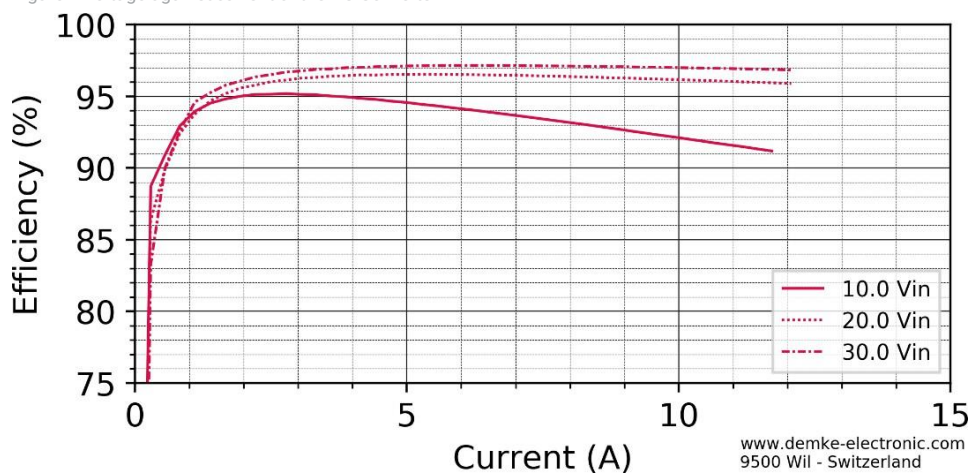
Figure 2 Efficiency in the constant voltage range of the DC-Converter
