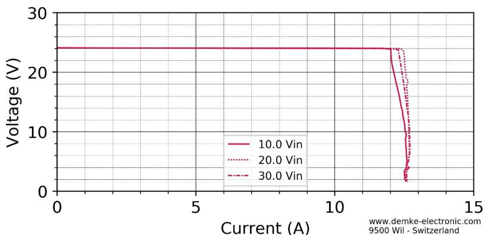
Figure 1 Voltage against current of the DC-Converter
