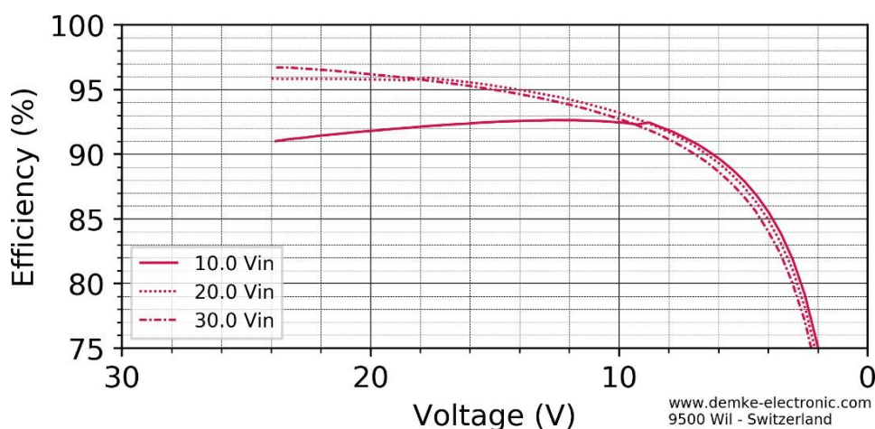
Figure 3 Efficiency in the constant current range of the DC-Converter
