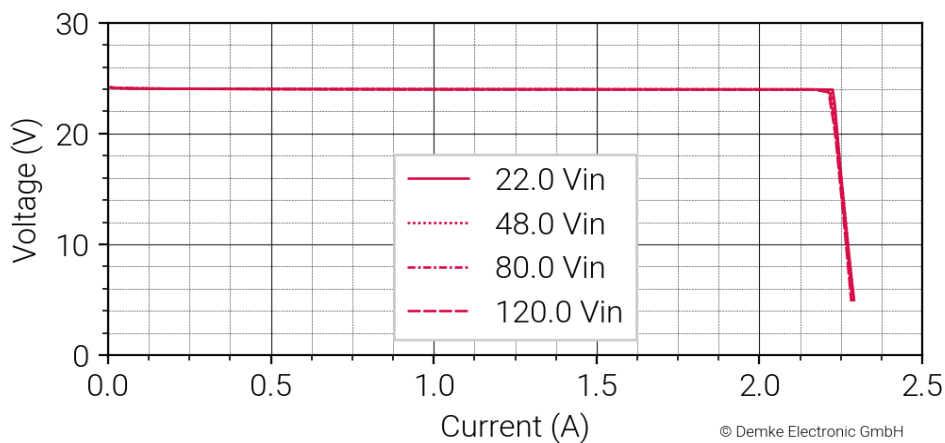
Figure 1 Voltage against current of the DC-Converter
