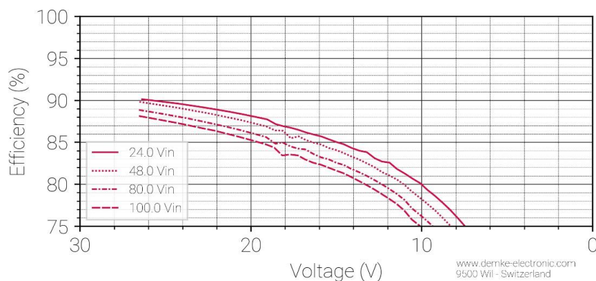
Figure 3 Efficiency in the constant current range of the DC-Converter
