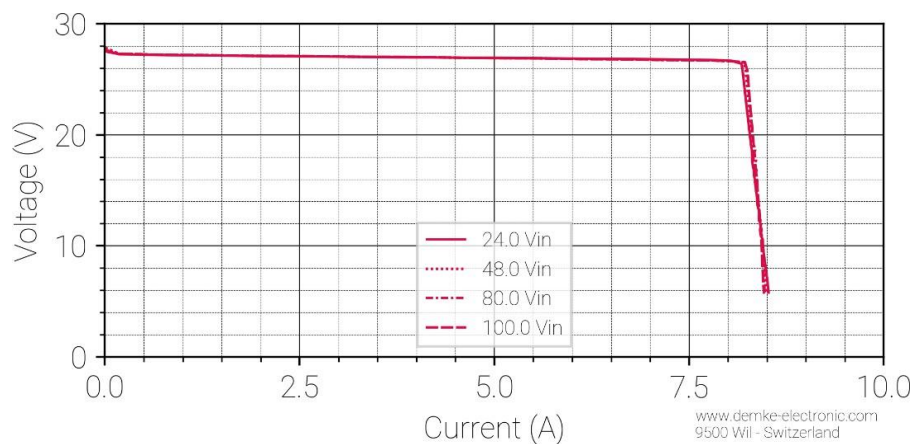
Figure 1 Voltage against current of the DC-Converter
