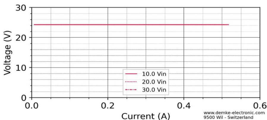
Figure 3 Voltage in CV-mode of the DC-Converter
