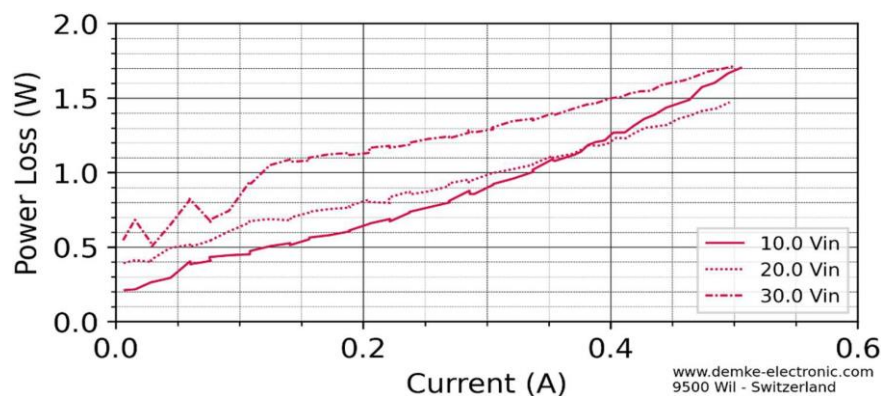
Figure 2 Power Loss over current of the DC-Converter
