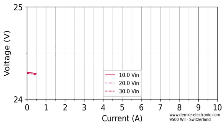
Figure 4 Voltage in CV-mode of the DC-Converter
