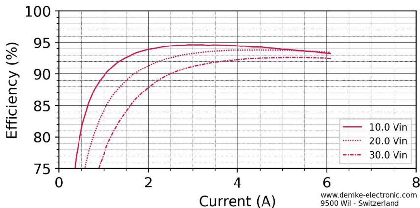
Figure 1 Efficiency in the constant voltage range of the DC-Converter
