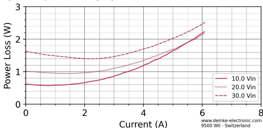
Figure 2 Power Loss over current of the DC-Converter
