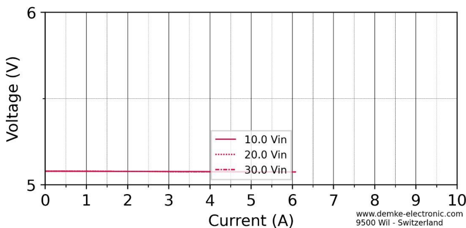
Figure 4 Voltage in CV-mode of the DC-Converter
