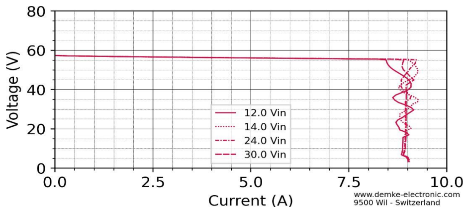
Figure 1 Voltage against current of the DC-Converter
