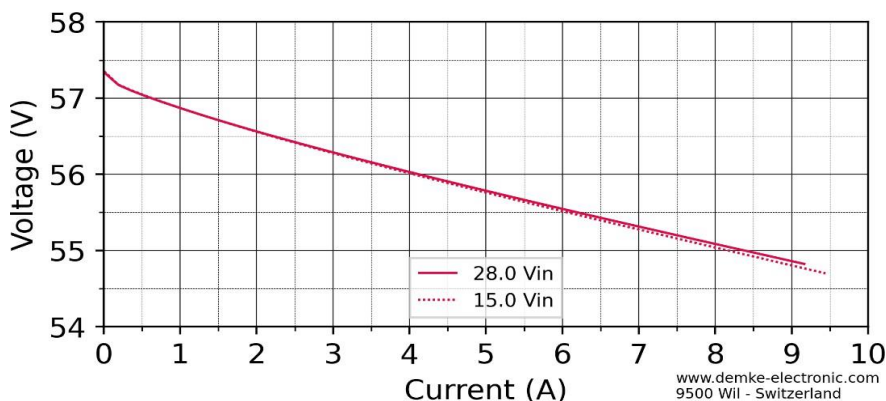
Figure 6: Output Voltage in CV-mode of the DC-Converter
