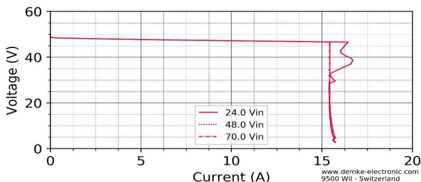
Figure 1 Voltage against current of the DC-Converter
