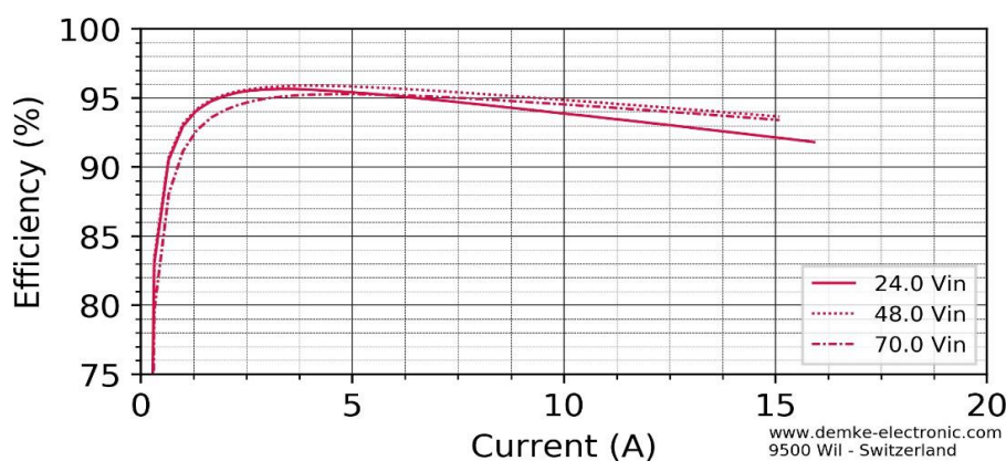
Figure 2 Efficiency in the constant voltage range of the DC-Converter
