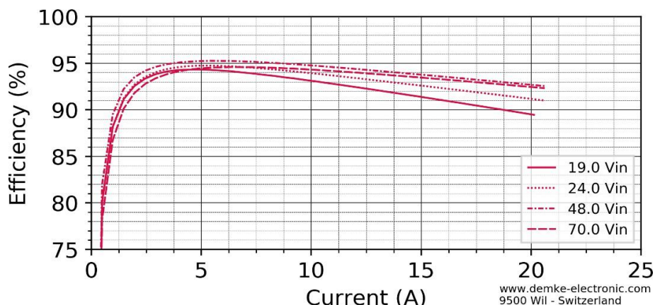
Figure 5: Efficiency in the constant voltage range of the DC-Converter in SH mode
