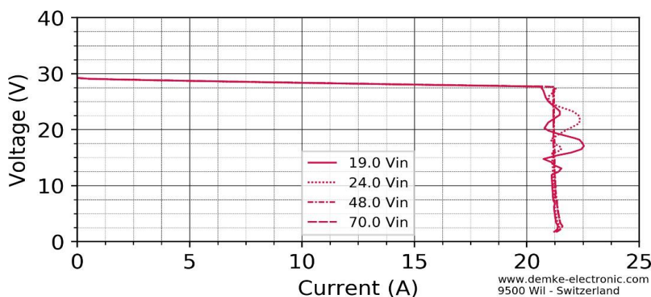
Figure 4: Voltage against current of the DC-Converter in SH mode
