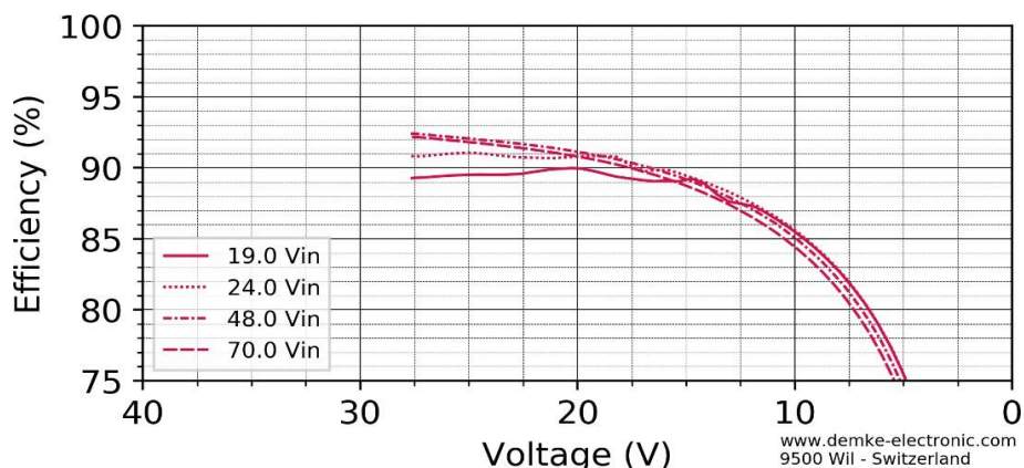
Figure 6: Efficiency in the constant current range of the DC-Converter 757-27-SD in SH mode
