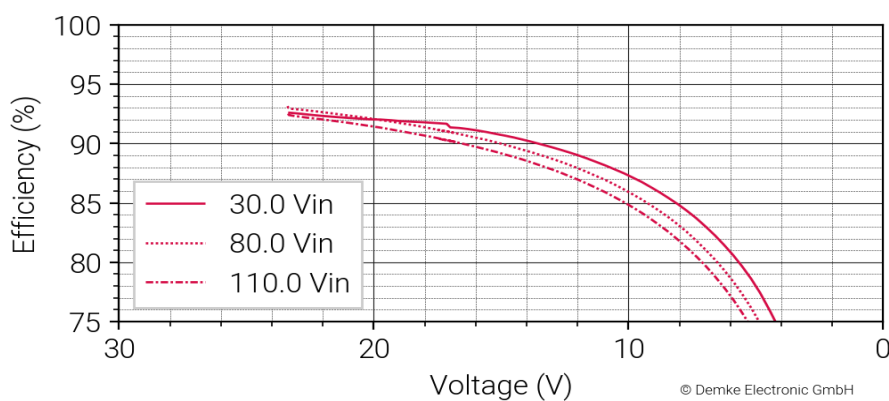
Figure 3 Efficiency in the constant current range of the DC-Converter
