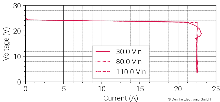
Figure 1 Voltage against current of the DC-Converter
