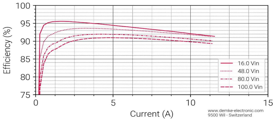
Figure 2 Efficiency in the constant voltage range of the DC-Converter
