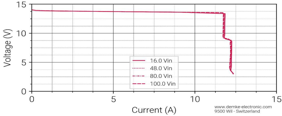
Figure 1 Voltage against current of the DC-Converter
