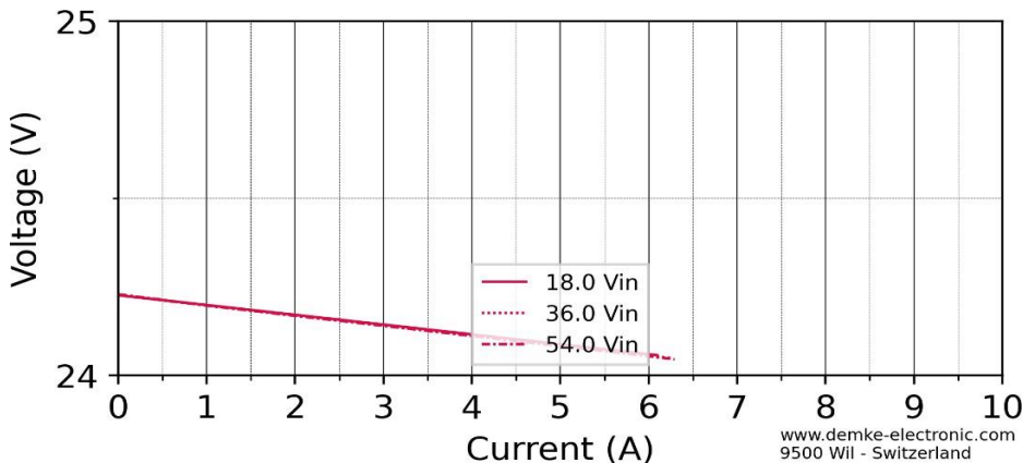
Figure 6: Voltage in CV-mode of the DC-Converter
