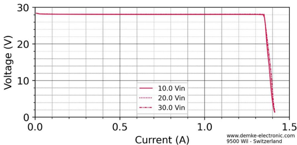
Figure 8: Switch-High Voltage against current of the DC-Converter
