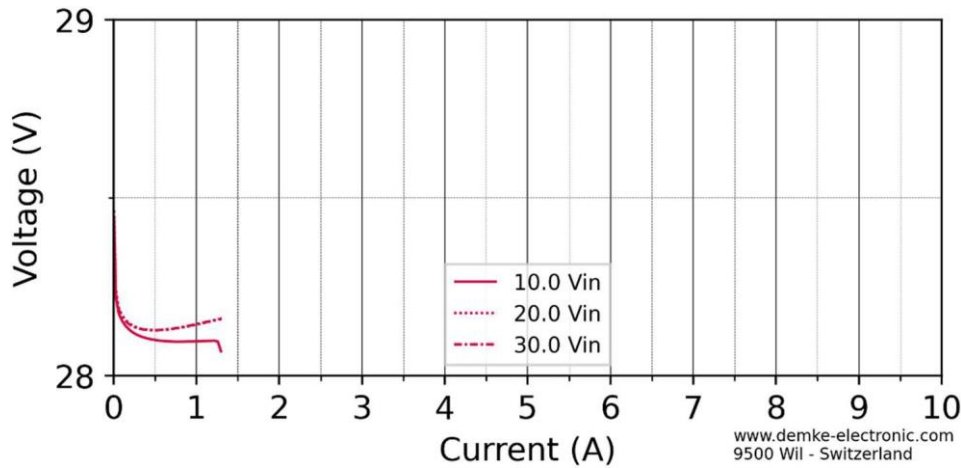
Figure 7: Switch-High voltage in CV-mode of the DC-Converter
