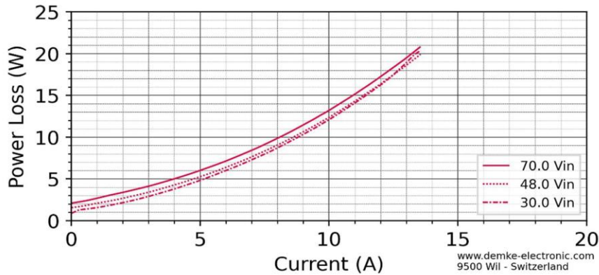
Figure 4: Power Loss over current of the DC-Converter
