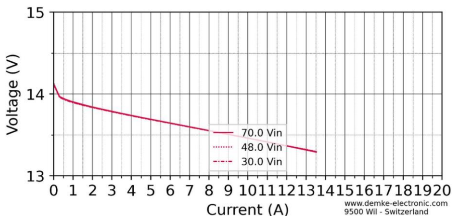
Figure 6: Voltage in CV-mode of the DC-Converter
