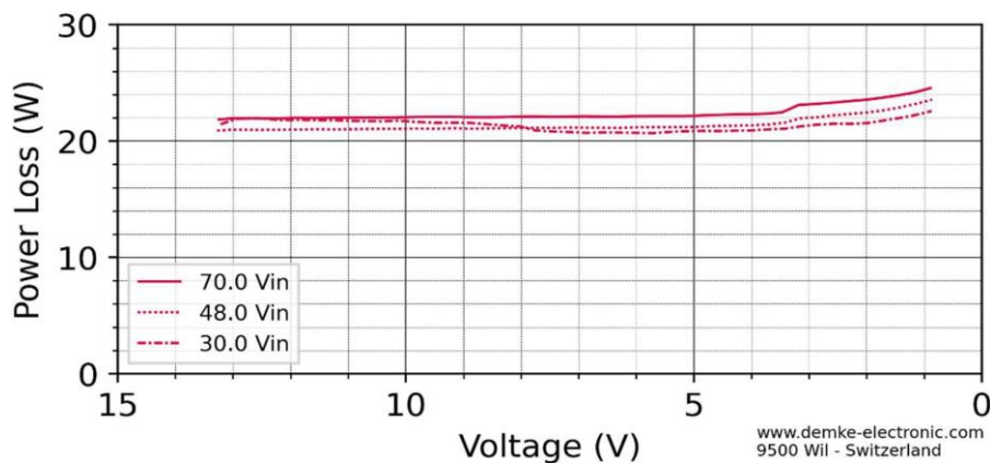
Figure 5: Power Loss over voltage of the DC-Converter
