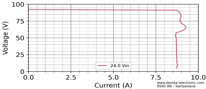
Figure 1 Voltage against current of the DC-Converter
