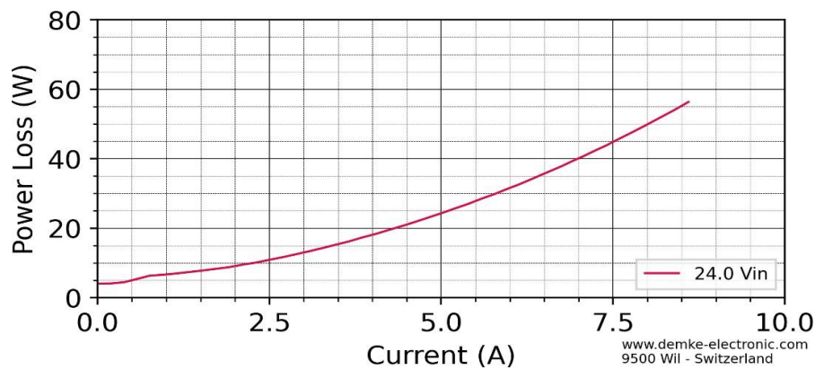
Figure 5: Power Loss over voltage of the DC-Converter
