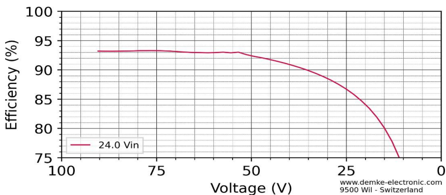
Figure 3 Efficiency in the constant current range of the DC Converter
