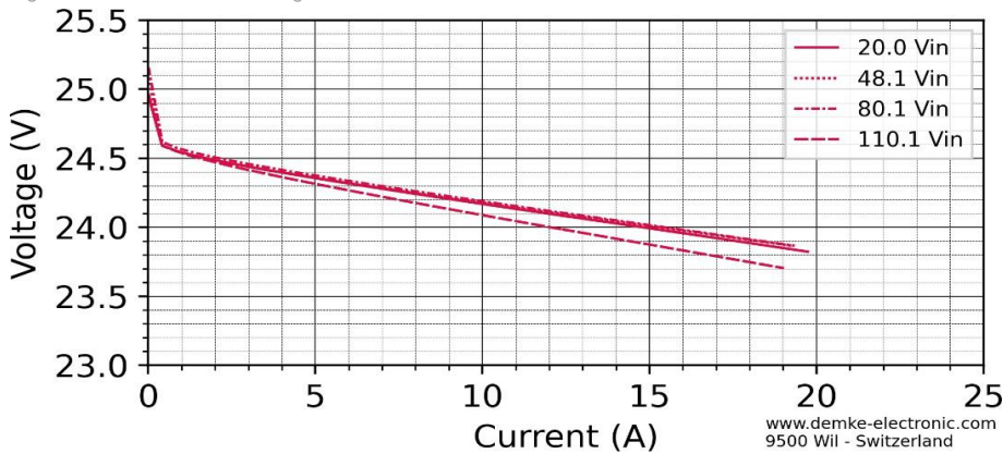
Figure 6: Voltage in CV-mode of the DC-Converter
