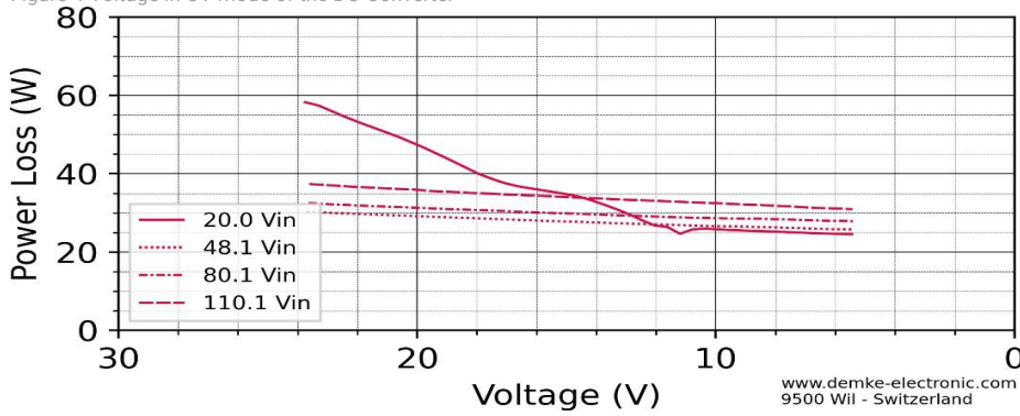
Figure 5: Power Loss over voltage of the DC-Converter
