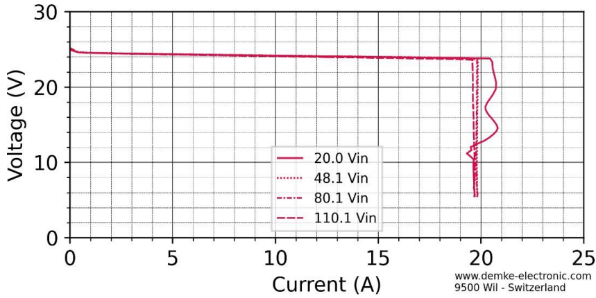
Figure 1 Voltage against current of the DC-Converter
