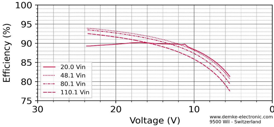
Figure 4 Voltage in CV-mode of the DC-Converter
